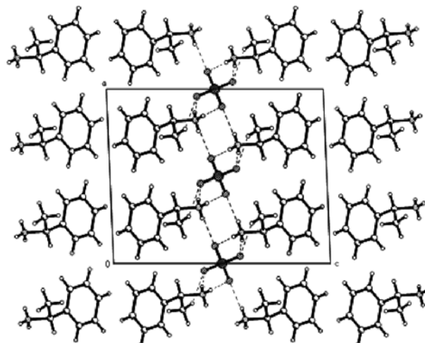
Fig. 2. Projection of molecule of compound II onto xOz plane. Hydrogen bonds are denoted with dashed lines.
